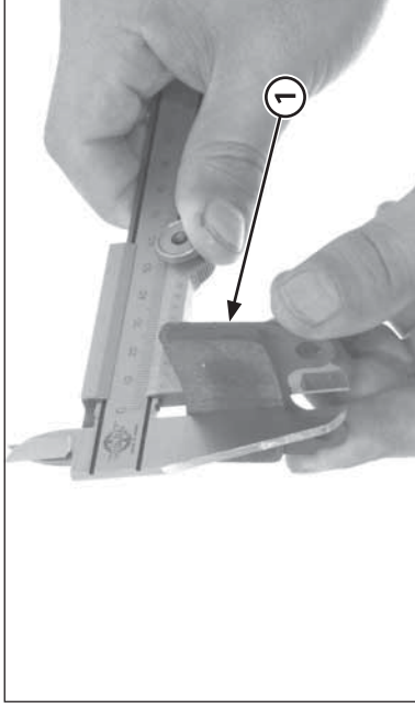
(1) BRAKE PAD
