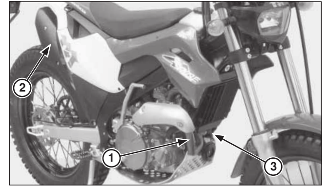
(1) EXHAUST PIPE (2) MUFFLER (3) LAMBDA-SONDE
