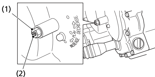
(1) lock nut
