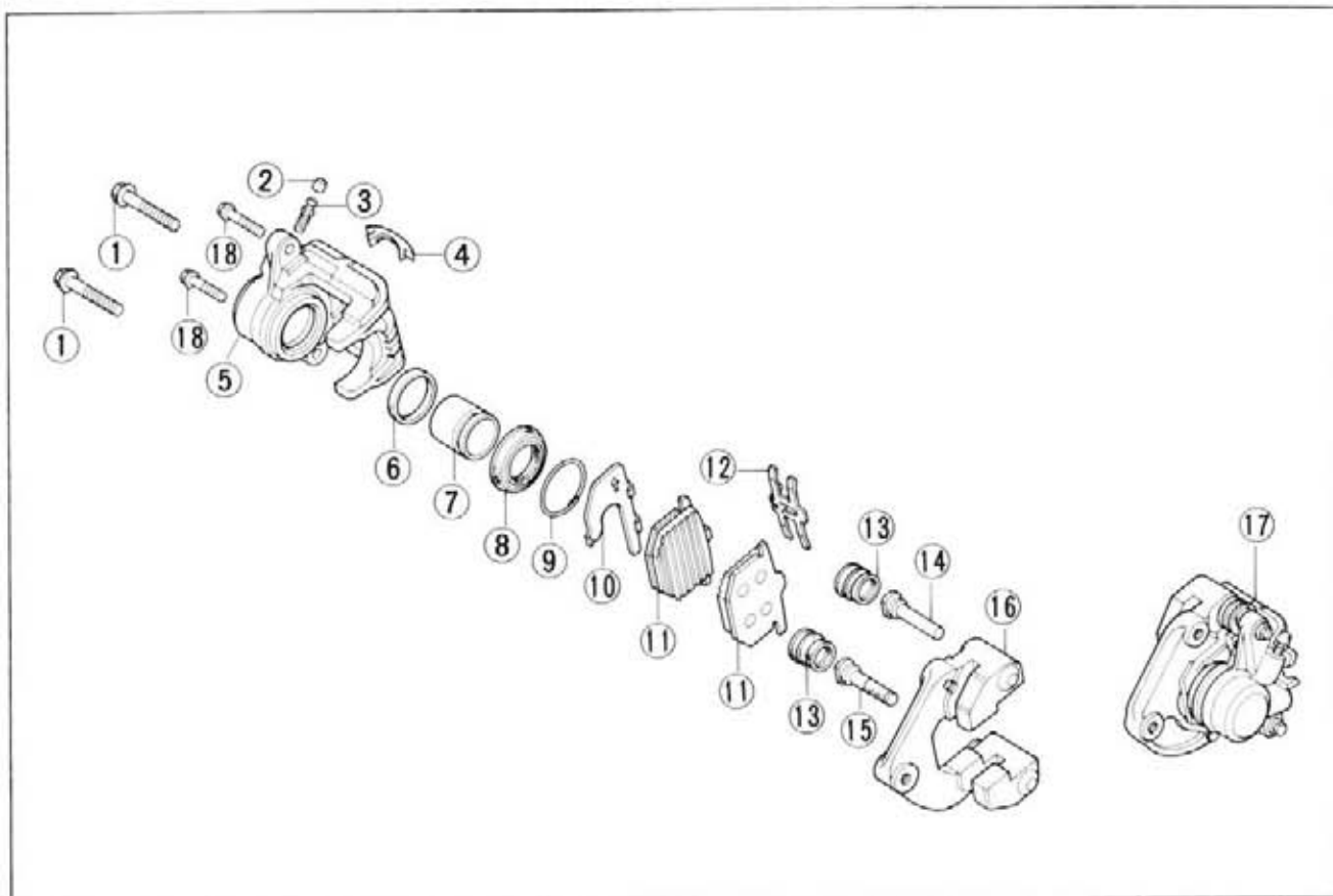
Fig. F2-1 ① Flange bolt (10×32) ⑥ Piston seal ⑪ Brake pad ⑯ Right bracket ② Bleed valve cap ⑦ Piston ⑫ Pad spring ⑰ Left caliper ③ Bleed valve ⑧ Piston boot ⑬ Dust cover assembly ④ Indicator cap ⑨ Piston boot clip ⑭ Pin A ⑱ 8mm flange bolt ⑤ Right caliper ⑩ Pad shim ⑮ Pin B
